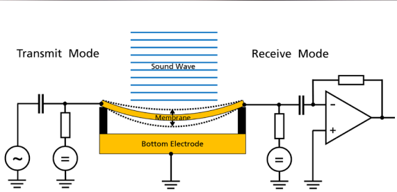
CMUT in transmit and receive mode
