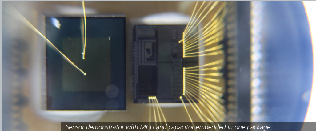
Sensor demonstrator with MCU and capacitor embedded in one package
