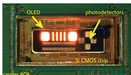
OLED-auf-Silizium Sensortest-Chip
